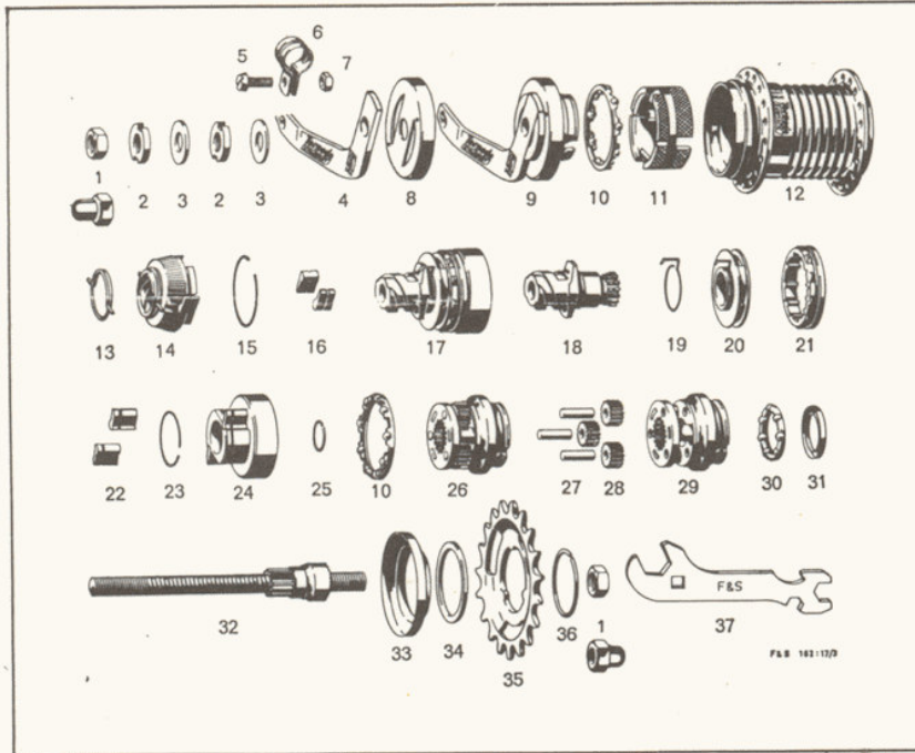
Spare Parts List for TORPEDO DUOMATIC Coaster Brake R 2110
